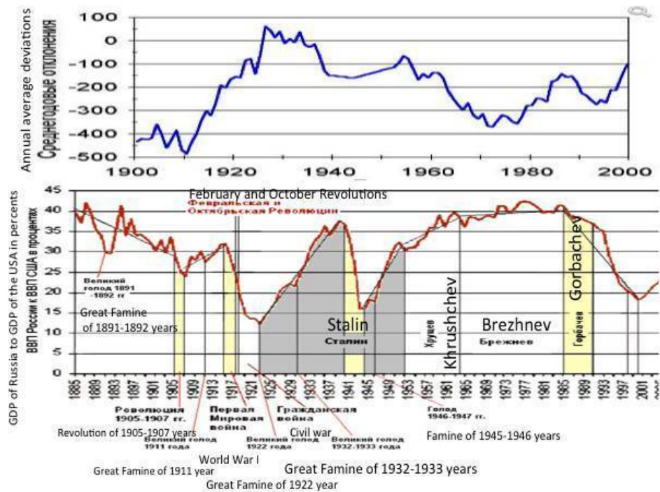
Correlation of the Earth's rotational velocity change and the relation between GDP of the USSR and Russia to the USA
