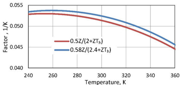
Figure. 7.3 Dependence of Figure-of-Merit on temperature.
