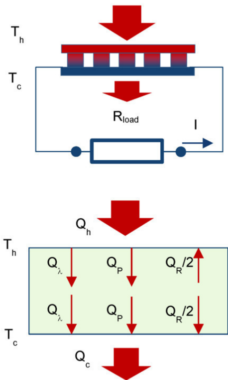
Figure. 2.2 Heat flow diagram for generating mode.
